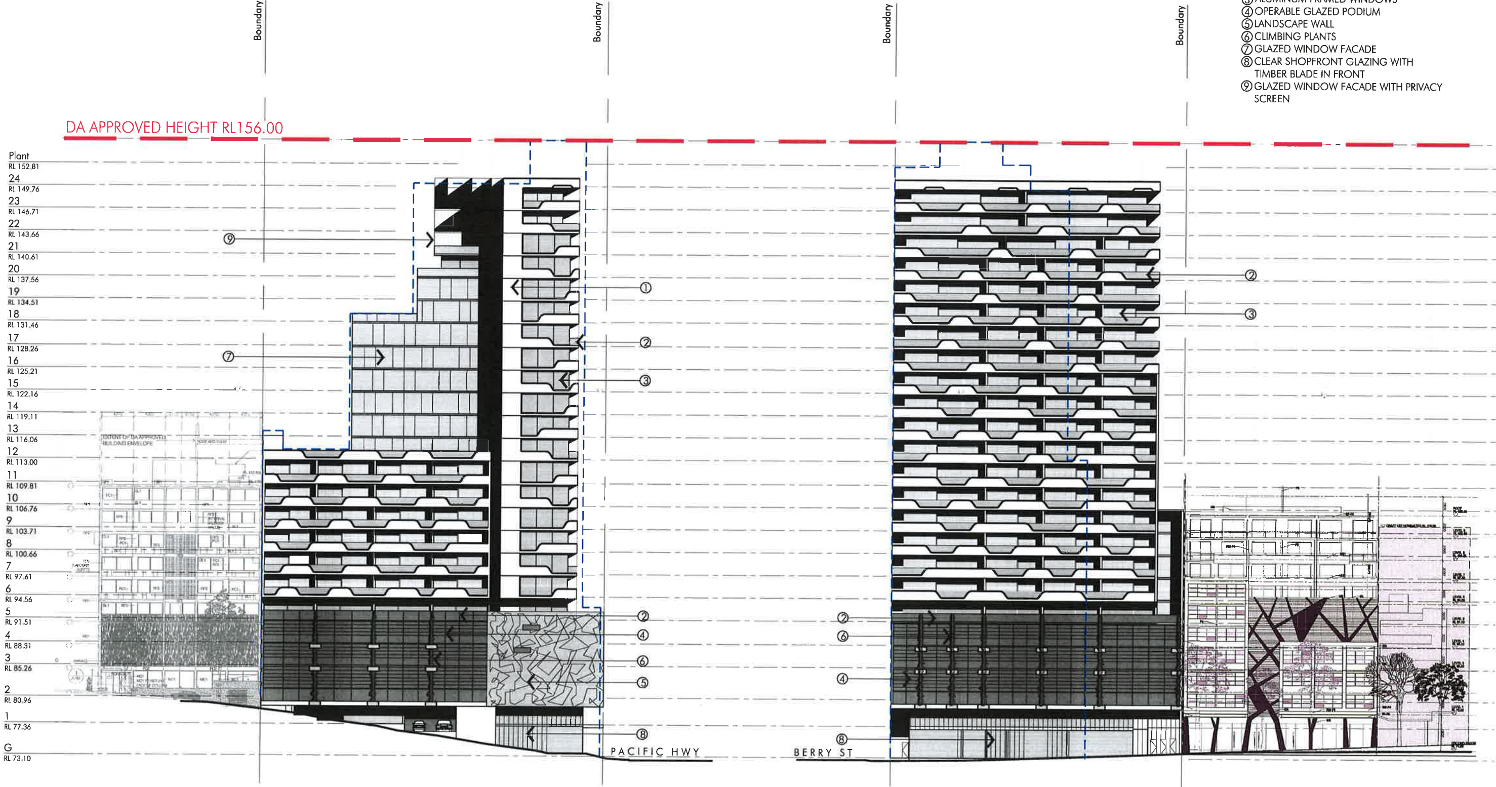
SOUTH ELEVATION - FACING BERRY ST
